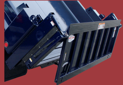
DUMP BODY - G2 SERIES
