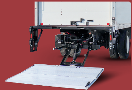
TUCKUNDER SERIES - TKL MODEL
